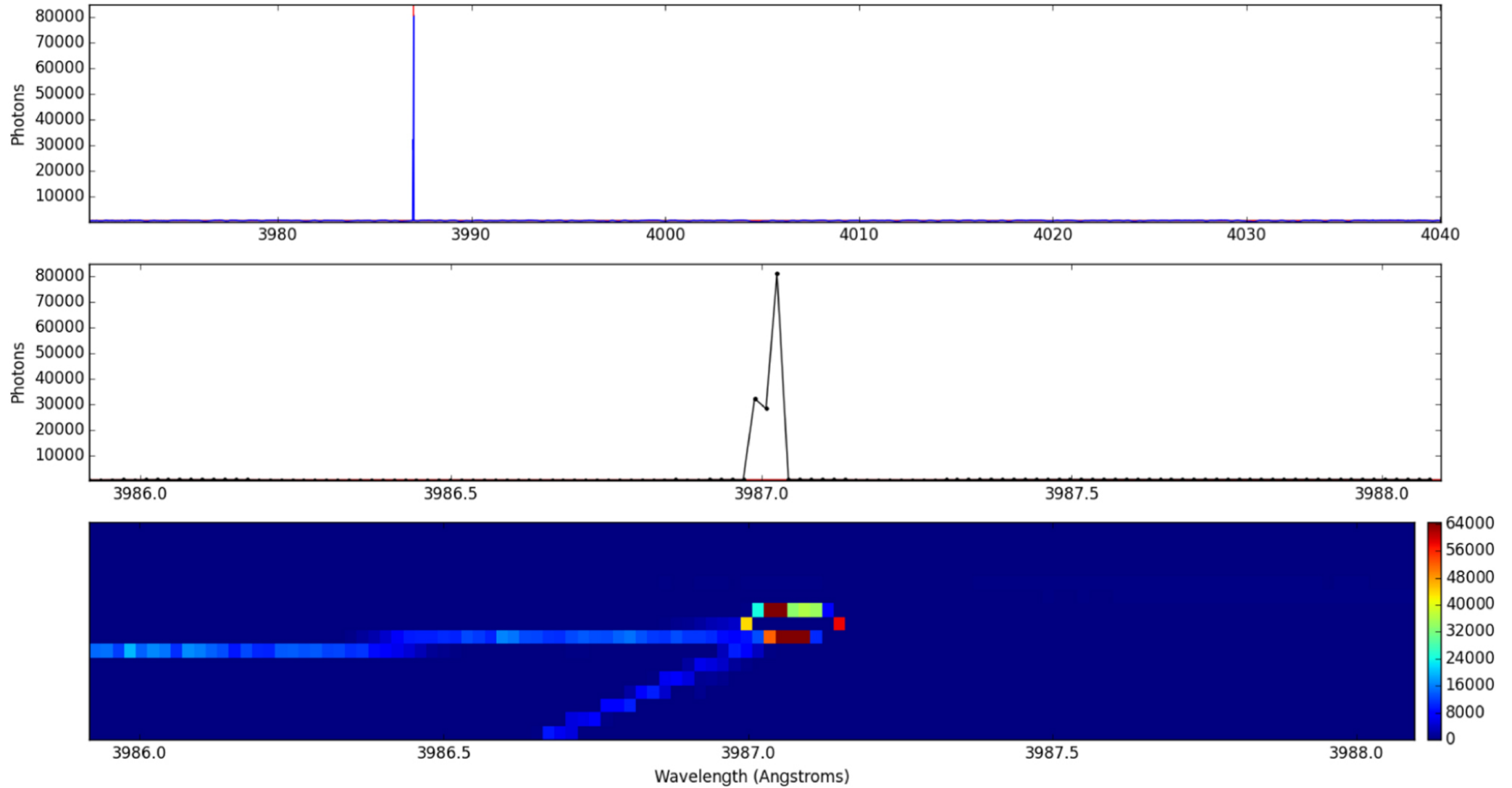
Figure 9. from A Search for Laser Emission with Megawatt Thresholds from 5600 FGKM Stars null 2017 AJ 153 251 doi:10.3847/1538-3881/aa6d12 https://dx.doi.org/10.3847/1538-3881/aa6d12 © 2017. The American Astronomical Society. All rights reserved.
