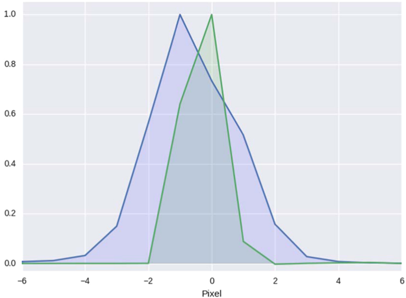
Figure 8. from A Search for Laser Emission with Megawatt Thresholds from 5600 FGKM Stars null 2017 AJ 153 251 doi:10.3847/1538-3881/aa6d12 https://dx.doi.org/10.3847/1538-3881/aa6d12 © 2017. The American Astronomical Society. All rights reserved.
