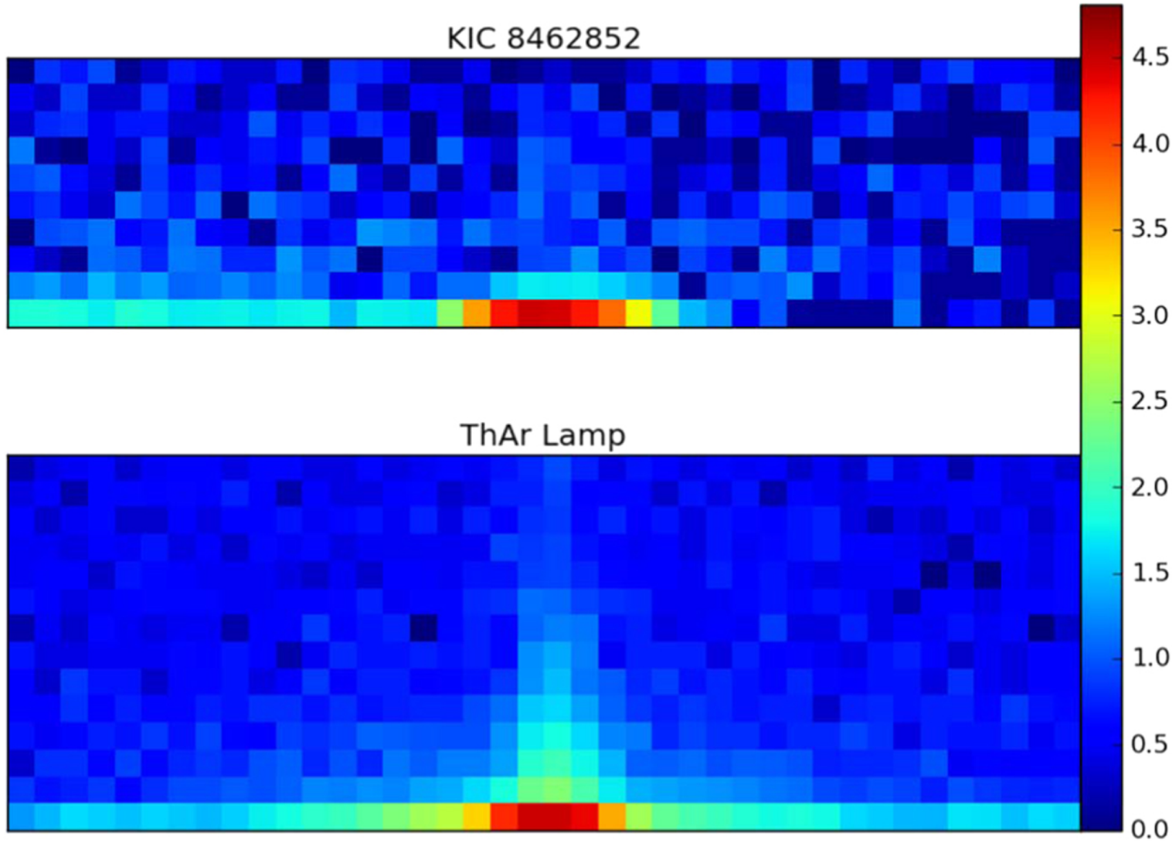
Figure 7. from A Search for Laser Emission with Megawatt Thresholds from 5600 FGKM Stars null 2017 AJ 153 251 doi:10.3847/1538-3881/aa6d12 https://dx.doi.org/10.3847/1538-3881/aa6d12 © 2017. The American Astronomical Society. All rights reserved.
