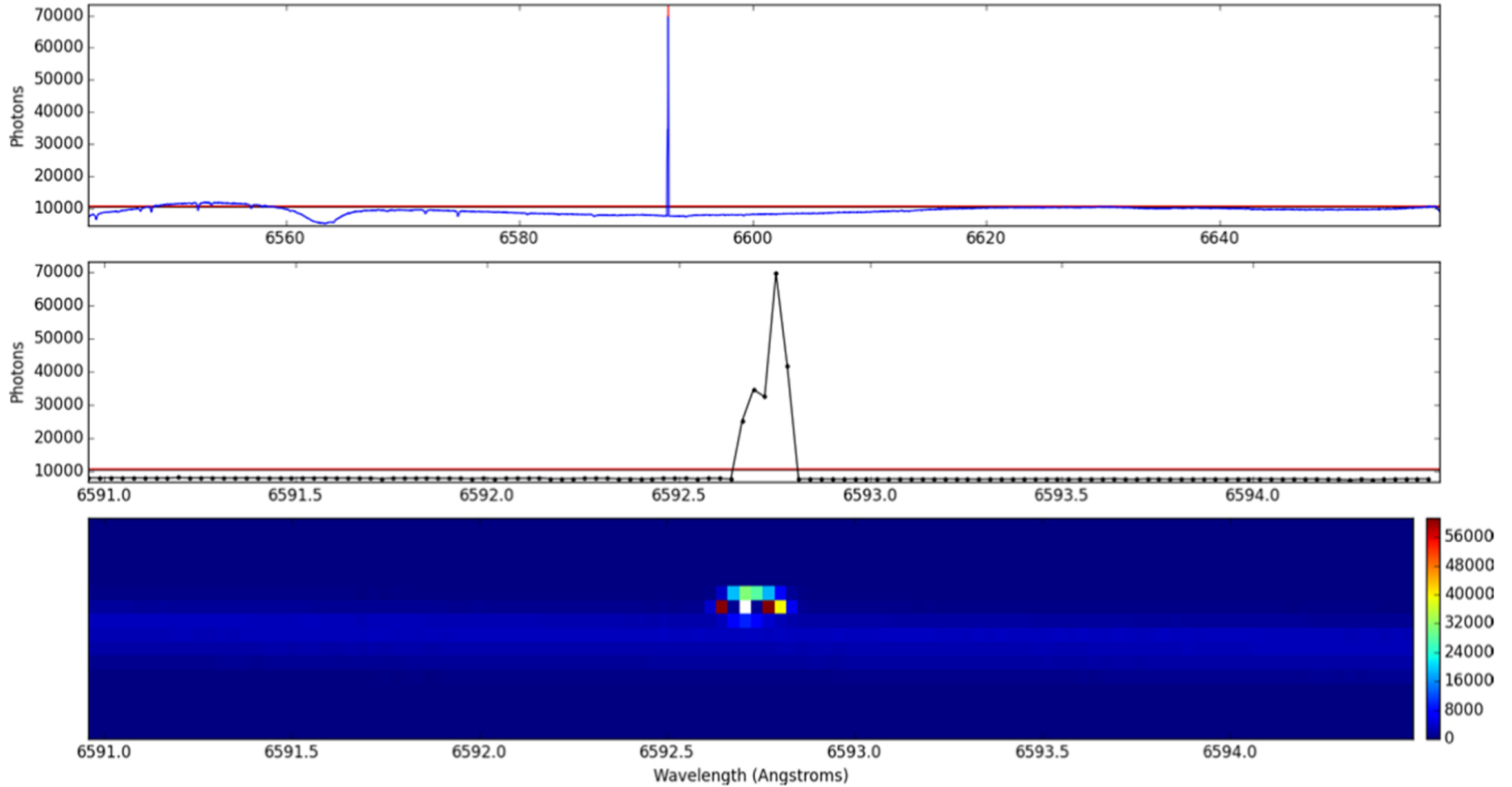
Figure 6. from A Search for Laser Emission with Megawatt Thresholds from 5600 FGKM Stars null 2017 AJ 153 251 doi:10.3847/1538-3881/aa6d12 https://dx.doi.org/10.3847/1538-3881/aa6d12 © 2017. The American Astronomical Society. All rights reserved.
