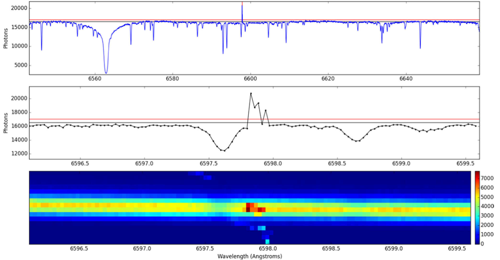
Figure 5. from A Search for Laser Emission with Megawatt Thresholds from 5600 FGKM Stars null 2017 AJ 153 251 doi:10.3847/1538-3881/aa6d12 https://dx.doi.org/10.3847/1538-3881/aa6d12 © 2017. The American Astronomical Society. All rights reserved.
