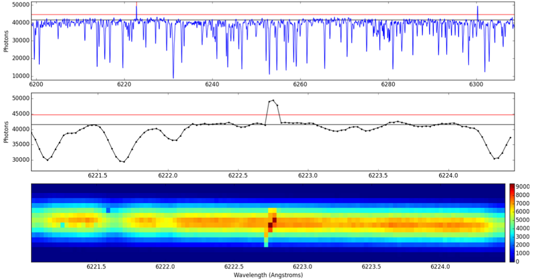
Figure 4. from A Search for Laser Emission with Megawatt Thresholds from 5600 FGKM Stars null 2017 AJ 153 251 doi:10.3847/1538-3881/aa6d12 https://dx.doi.org/10.3847/1538-3881/aa6d12 © 2017. The American Astronomical Society. All rights reserved.
