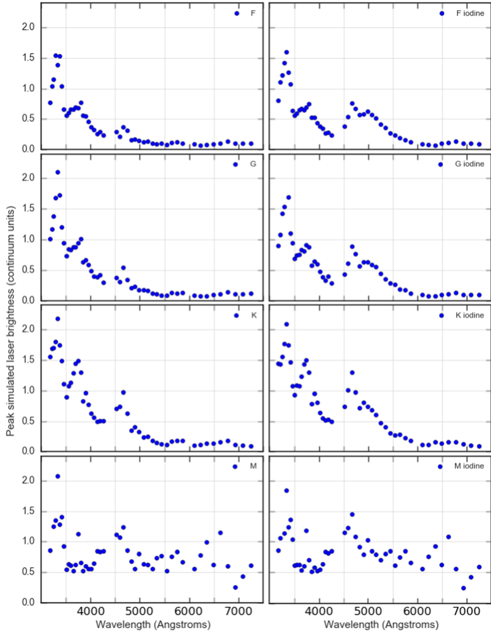
Figure 3. from A Search for Laser Emission with Megawatt Thresholds from 5600 FGKM Stars null 2017 AJ 153 251 doi:10.3847/1538-3881/aa6d12 https://dx.doi.org/10.3847/1538-3881/aa6d12 © 2017. The American Astronomical Society. All rights reserved.
