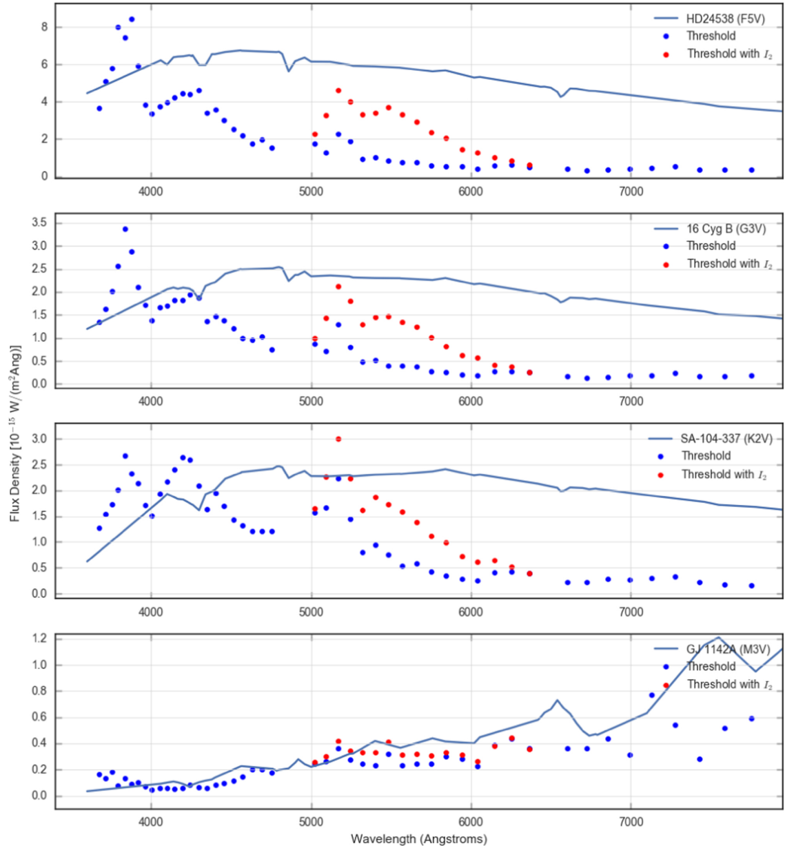
Figure 15. from A Search for Laser Emission with Megawatt Thresholds from 5600 FGKM Stars null 2017 AJ 153 251 doi:10.3847/1538-3881/aa6d12 https://dx.doi.org/10.3847/1538-3881/aa6d12 © 2017. The American Astronomical Society. All rights reserved.
