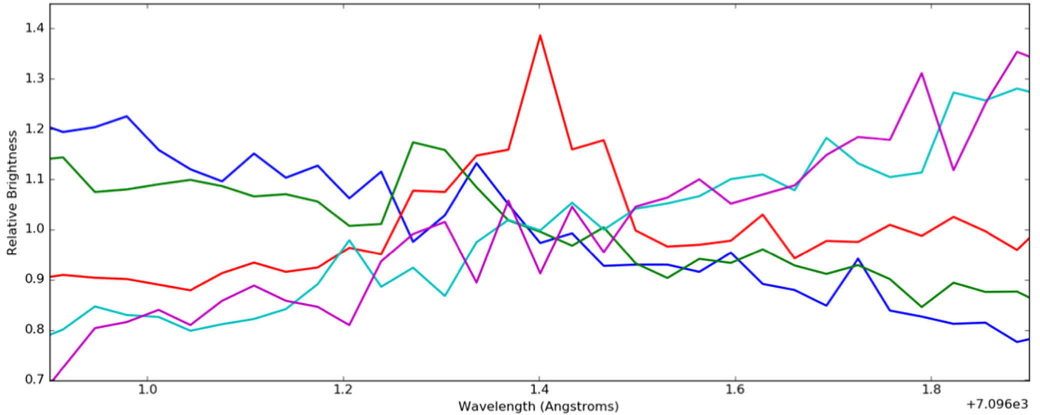
Figure 14. from A Search for Laser Emission with Megawatt Thresholds from 5600 FGKM Stars null 2017 AJ 153 251 doi:10.3847/1538-3881/aa6d12 https://dx.doi.org/10.3847/1538-3881/aa6d12 © 2017. The American Astronomical Society. All rights reserved.
