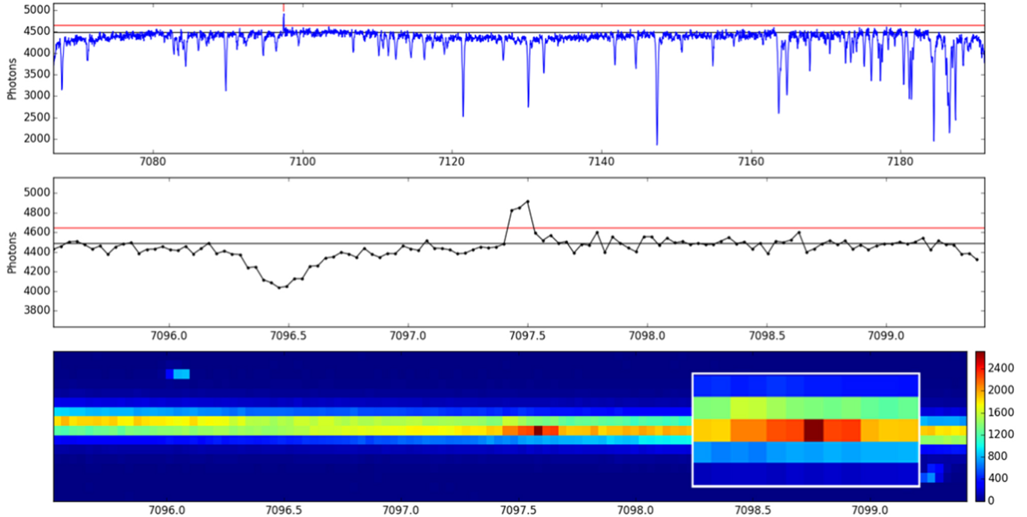
Figure 13. from A Search for Laser Emission with Megawatt Thresholds from 5600 FGKM Stars null 2017 AJ 153 251 doi:10.3847/1538-3881/aa6d12 https://dx.doi.org/10.3847/1538-3881/aa6d12 © 2017. The American Astronomical Society. All rights reserved.
