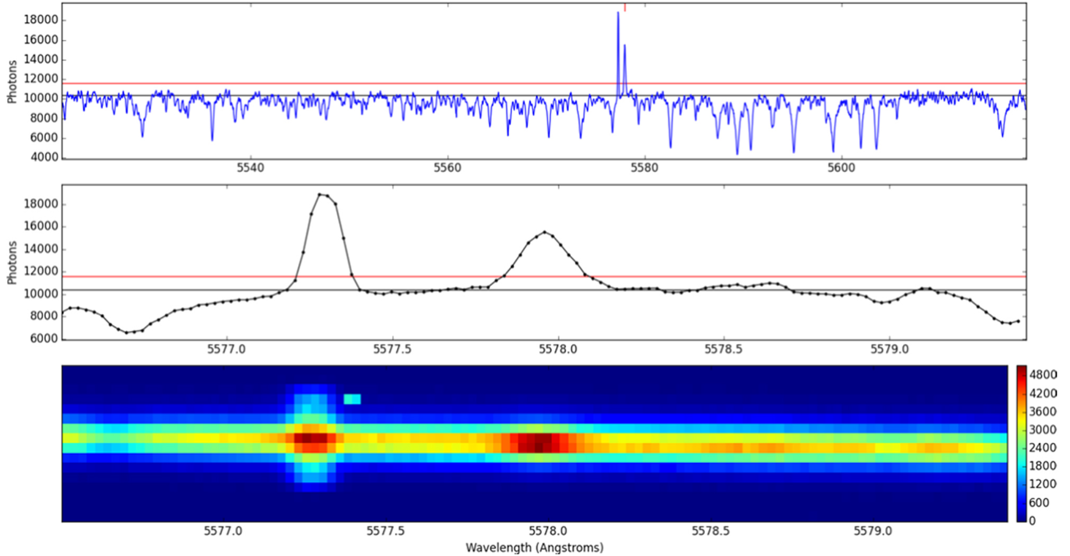
Figure 12. from A Search for Laser Emission with Megawatt Thresholds from 5600 FGKM Stars null 2017 AJ 153 251 doi:10.3847/1538-3881/aa6d12 https://dx.doi.org/10.3847/1538-3881/aa6d12 © 2017. The American Astronomical Society. All rights reserved.
