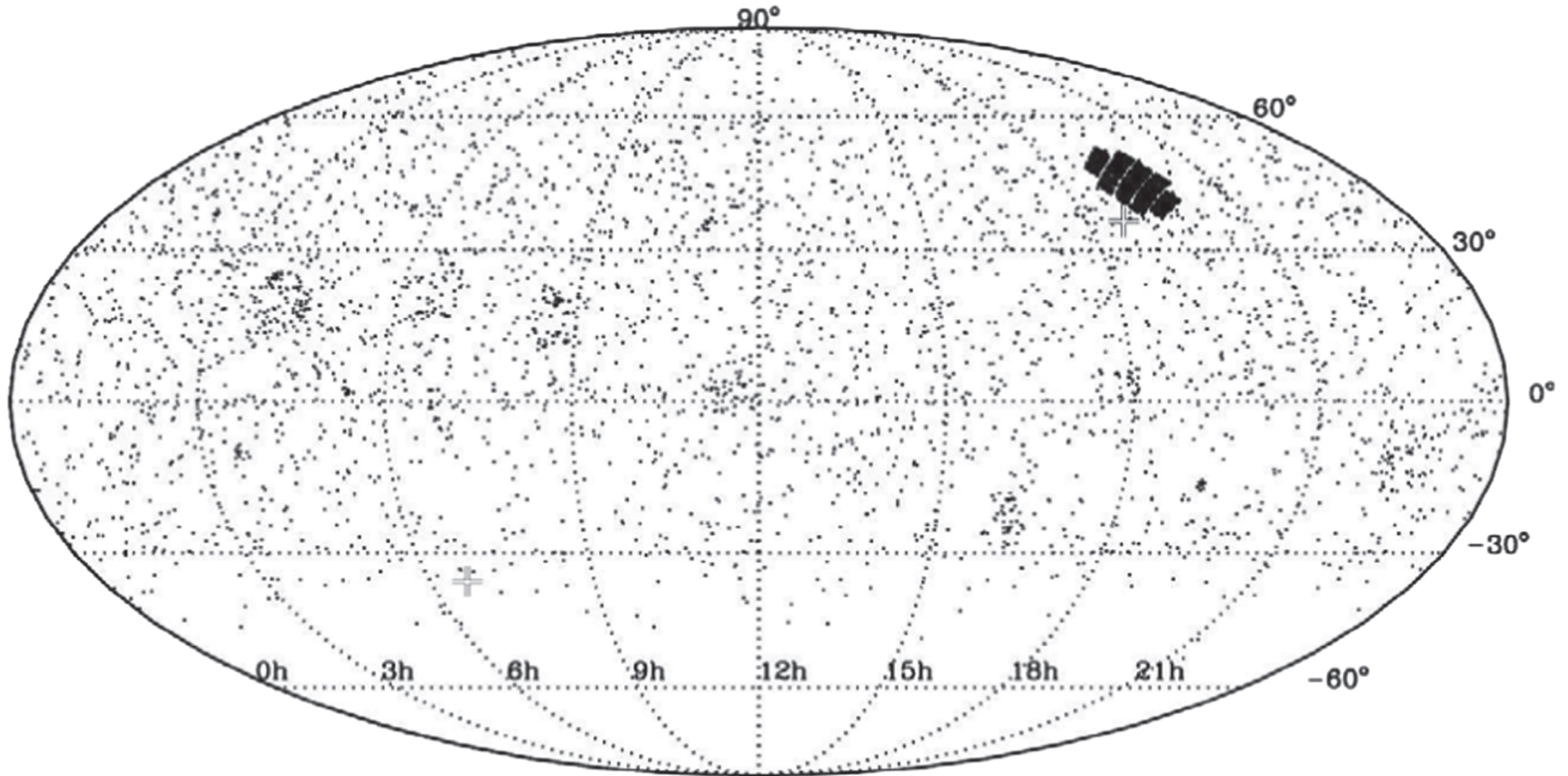
Figure 1. from A Search for Laser Emission with Megawatt Thresholds from 5600 FGKM Stars null 2017 AJ 153 251 doi:10.3847/1538-3881/aa6d12 https://dx.doi.org/10.3847/1538-3881/aa6d12 © 2017. The American Astronomical Society. All rights reserved.
