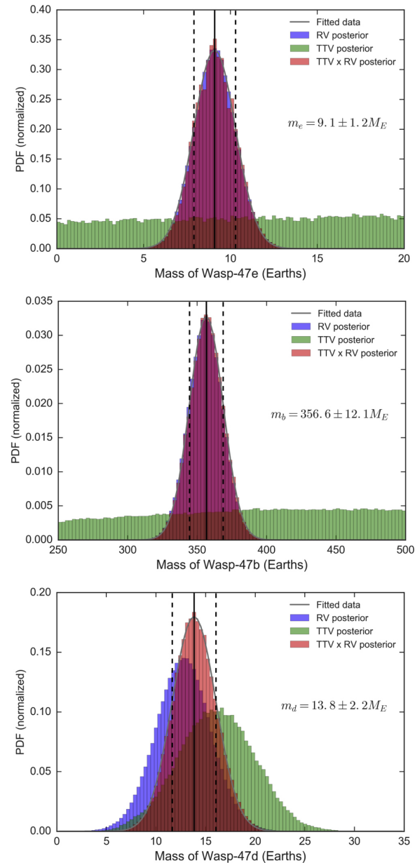
Figure 7. from New Insights on Planet Formation in WASP-47 from a Simultaneous Analysis of Radial Velocities and Transit Timing Variations null 2017 AJ 153 265 doi:10.3847/1538-3881/aa6c29 https://dx.doi.org/10.3847/1538-3881/aa6c29 © 2017. The American Astronomical Society. All rights reserved.
