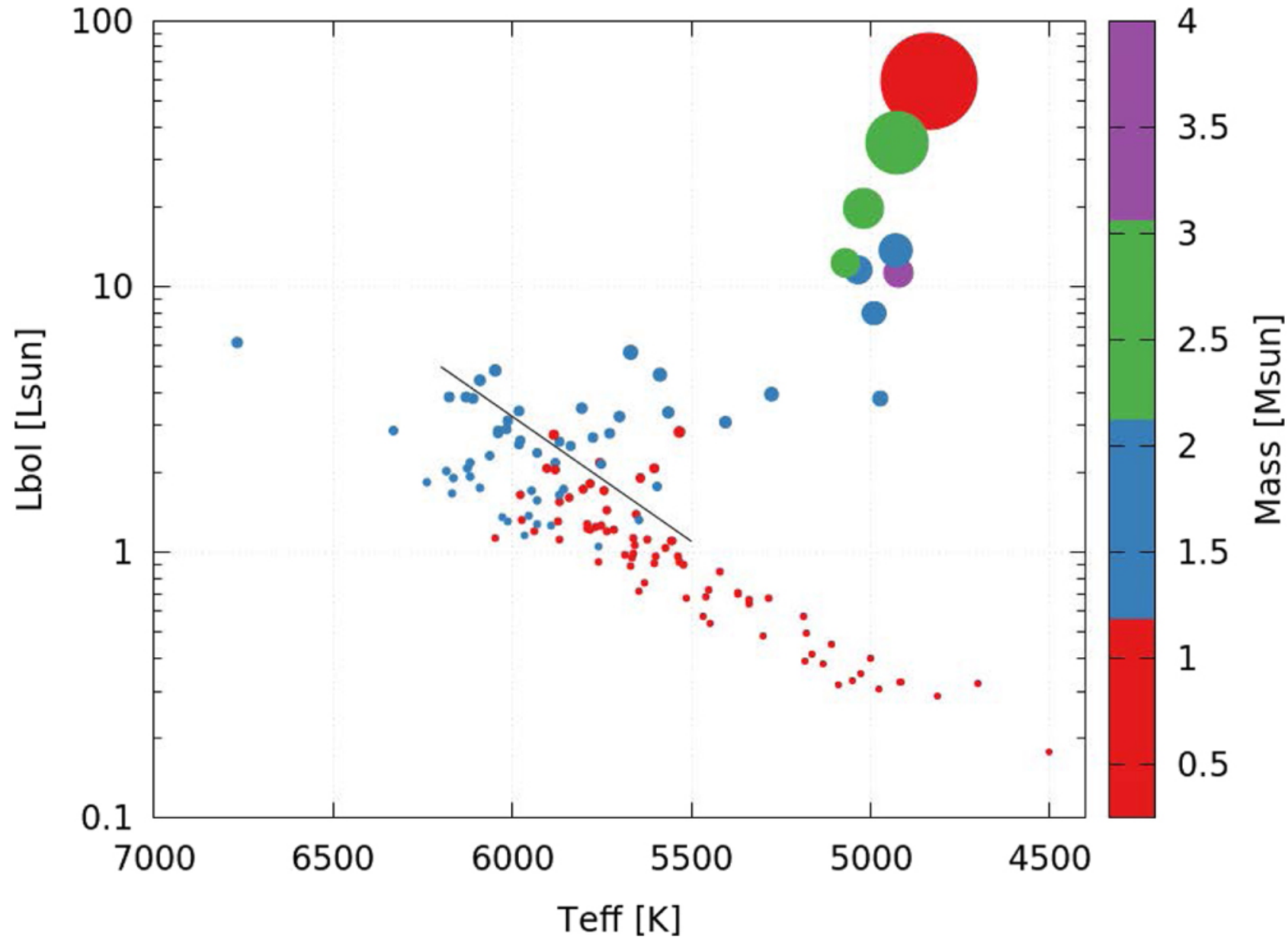
Figure 13. from Accurate Empirical Radii and Masses of Planets and Their Host Stars with Gaia Parallaxes null 2017 AJ 153 136 doi:10.3847/1538-3881/aa5df3 https://dx.doi.org/10.3847/1538-3881/aa5df3 © 2017. The American Astronomical Society. All rights reserved.
