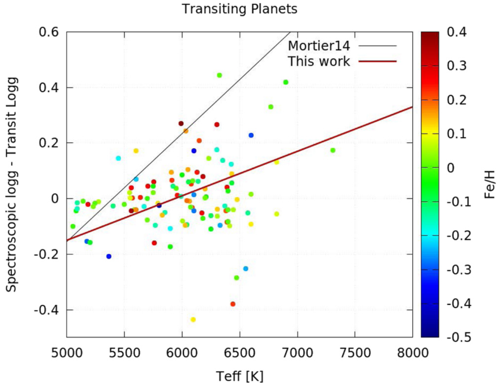
Figure 10. from Accurate Empirical Radii and Masses of Planets and Their Host Stars with Gaia Parallaxes null 2017 AJ 153 136 doi:10.3847/1538-3881/aa5df3 https://dx.doi.org/10.3847/1538-3881/aa5df3 © 2017. The American Astronomical Society. All rights reserved.
