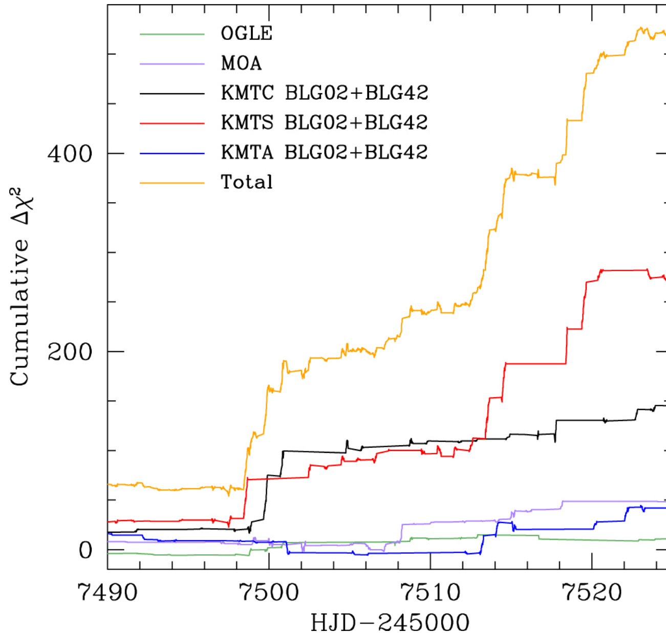
Figure 6. from Binary Source Microlensing Event OGLE-2016-BLG-0733: Interpretation of a Long-term Asymmetric Perturbation null 2017 AJ 153 129 doi:10.3847/1538-3881/aa5d07 https://dx.doi.org/10.3847/1538-3881/aa5d07 © 2017. The American Astronomical Society. All rights reserved.
