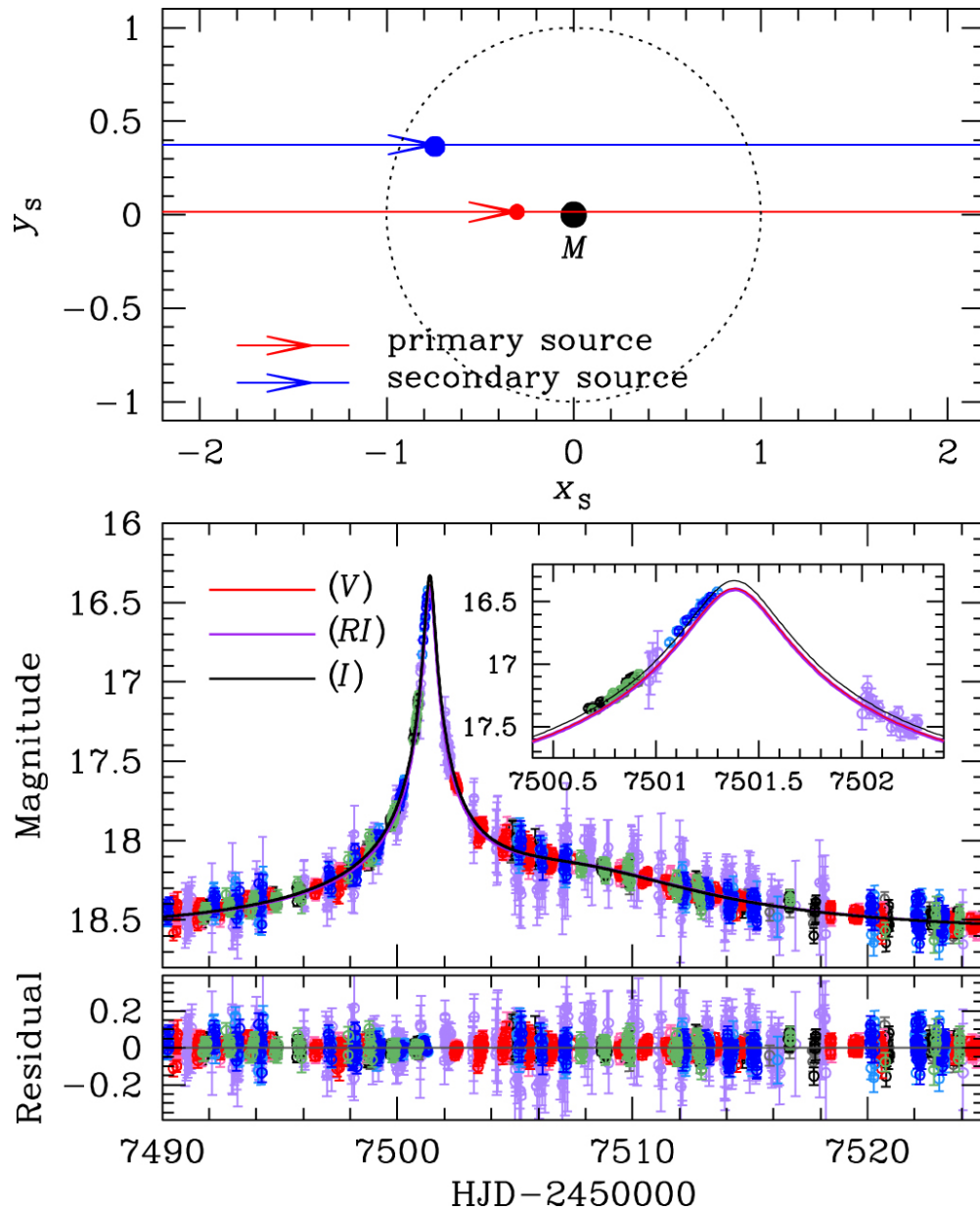
Figure 5. from Binary Source Microlensing Event OGLE-2016-BLG-0733: Interpretation of a Long-term Asymmetric Perturbation null 2017 AJ 153 129 doi:10.3847/1538-3881/aa5d07 https://dx.doi.org/10.3847/1538-3881/aa5d07 © 2017. The American Astronomical Society. All rights reserved.
