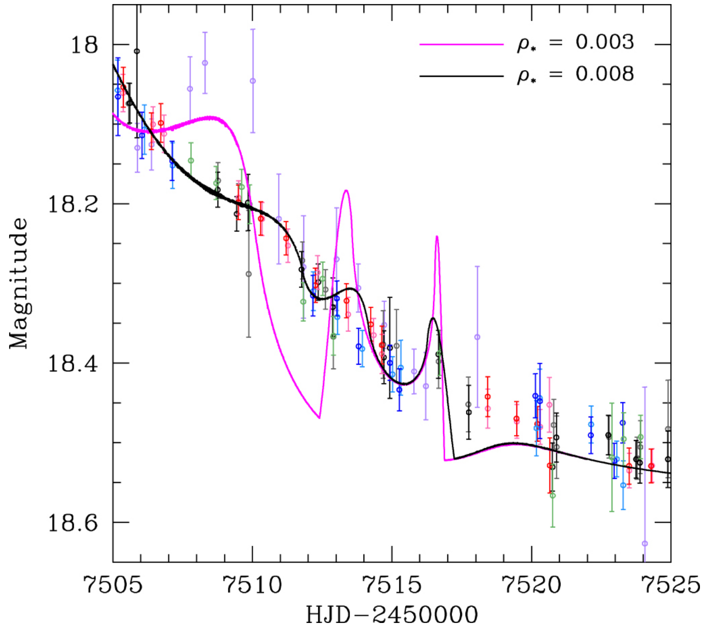
Figure 4. from Binary Source Microlensing Event OGLE-2016-BLG-0733: Interpretation of a Long-term Asymmetric Perturbation null 2017 AJ 153 129 doi:10.3847/1538-3881/aa5d07 https://dx.doi.org/10.3847/1538-3881/aa5d07 © 2017. The American Astronomical Society. All rights reserved.
