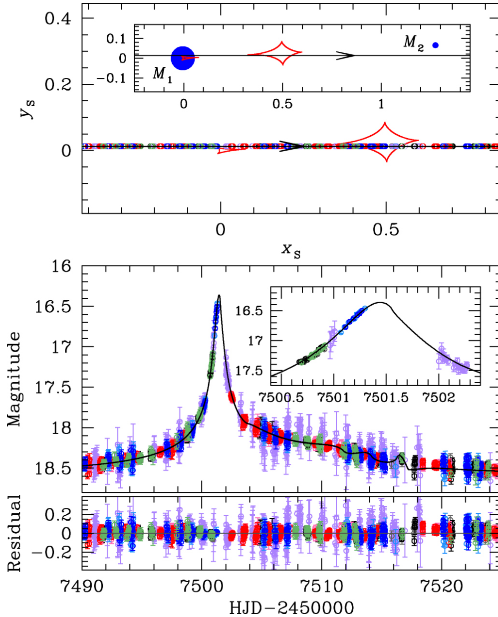
Figure 3. from Binary Source Microlensing Event OGLE-2016-BLG-0733: Interpretation of a Long-term Asymmetric Perturbation null 2017 AJ 153 129 doi:10.3847/1538-3881/aa5d07 https://dx.doi.org/10.3847/1538-3881/aa5d07
