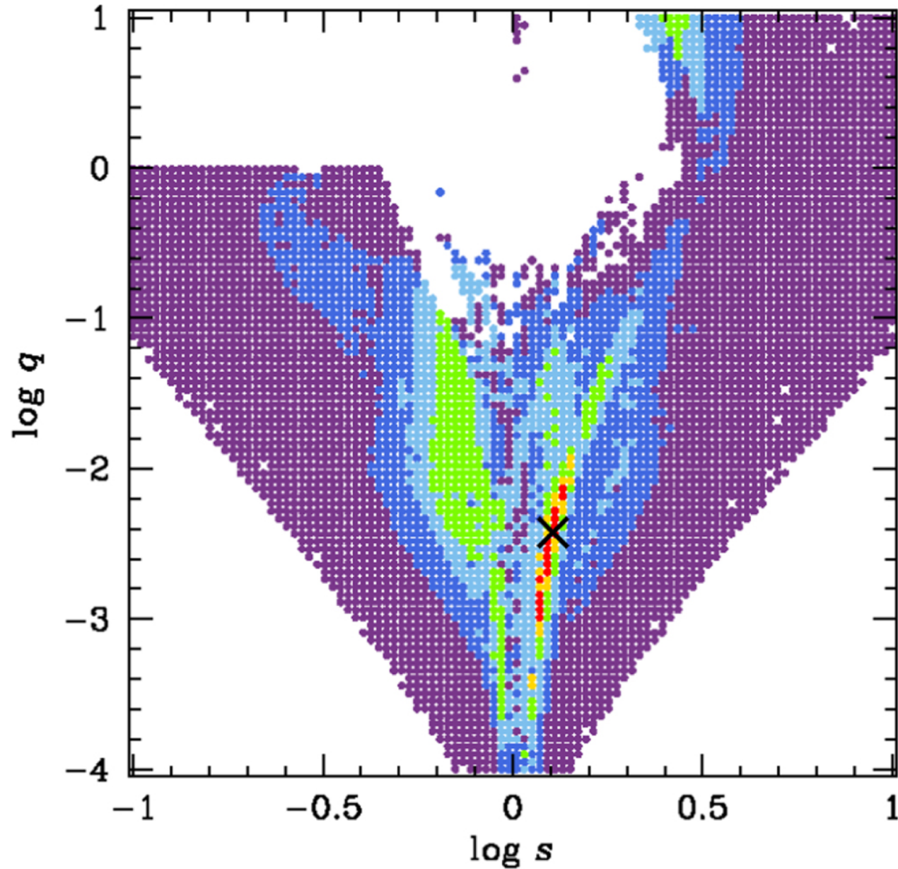
Figure 2. from Binary Source Microlensing Event OGLE-2016-BLG-0733: Interpretation of a Long-term Asymmetric Perturbation null 2017 AJ 153 129 doi:10.3847/1538-3881/aa5d07 https://dx.doi.org/10.3847/1538-3881/aa5d07 © 2017. The American Astronomical Society. All rights reserved.
