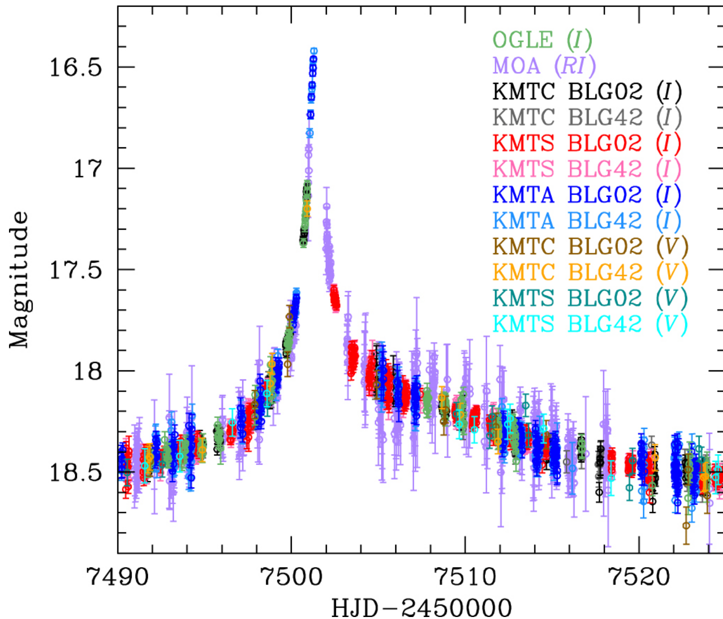
Figure 1. from Binary Source Microlensing Event OGLE-2016-BLG-0733: Interpretation of a Long-term Asymmetric Perturbation null 2017 AJ 153 129 doi:10.3847/1538-3881/aa5d07 https://dx.doi.org/10.3847/1538-3881/aa5d07 © 2017. The American Astronomical Society. All rights reserved.
