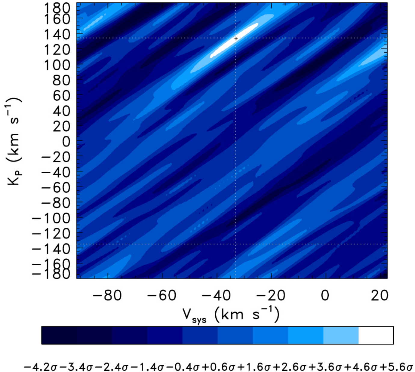
Figure 8. from Discovery of Water at High Spectral Resolution in the Atmosphere of 51 Peg b null 2017 AJ 153 138 doi:10.3847/1538-3881/aa5c87 https://dx.doi.org/10.3847/1538-3881/aa5c87 © 2017. The American Astronomical Society. All rights reserved.
