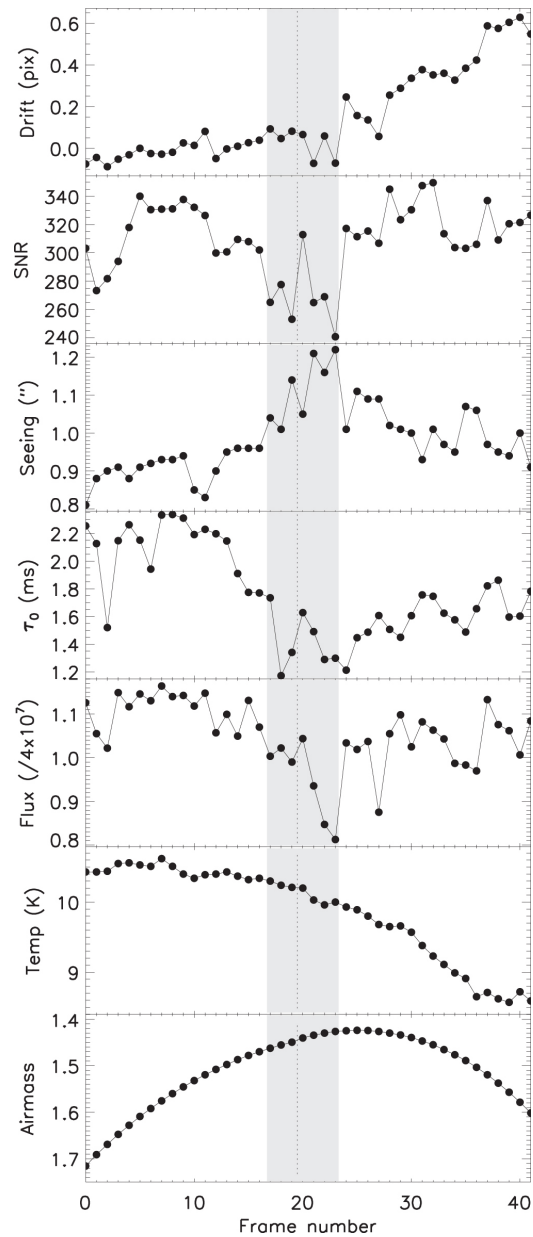
Figure 5. from Discovery of Water at High Spectral Resolution in the Atmosphere of 51 Peg b null 2017 AJ 153 138 doi:10.3847/1538-3881/aa5c87 https://dx.doi.org/10.3847/1538-3881/aa5c87 © 2017. The American Astronomical Society. All rights reserved.
