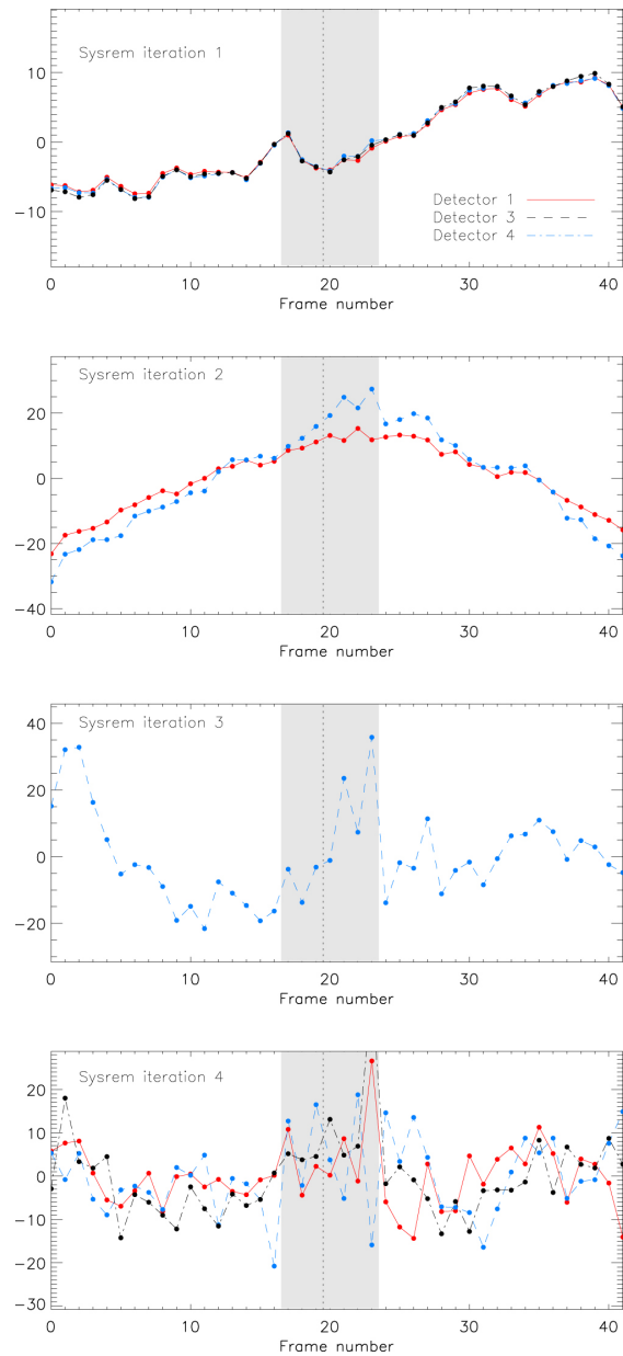
Figure 4. from Discovery of Water at High Spectral Resolution in the Atmosphere of 51 Peg b null 2017 AJ 153 138 doi:10.3847/1538-3881/aa5c87 https://dx.doi.org/10.3847/1538-3881/aa5c87 © 2017. The American Astronomical Society. All rights reserved.
