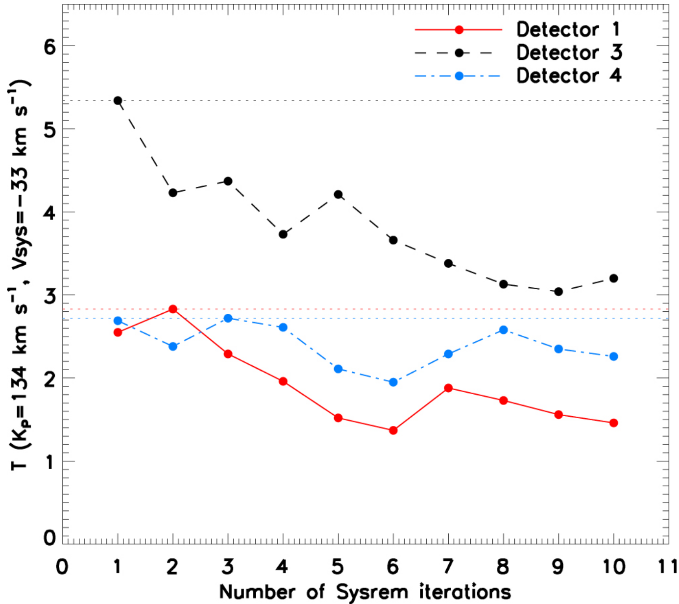
Figure 3. from Discovery of Water at High Spectral Resolution in the Atmosphere of 51 Peg b null 2017 AJ 153 138 doi:10.3847/1538-3881/aa5c87 https://dx.doi.org/10.3847/1538-3881/aa5c87 © 2017. The American Astronomical Society. All rights reserved.
