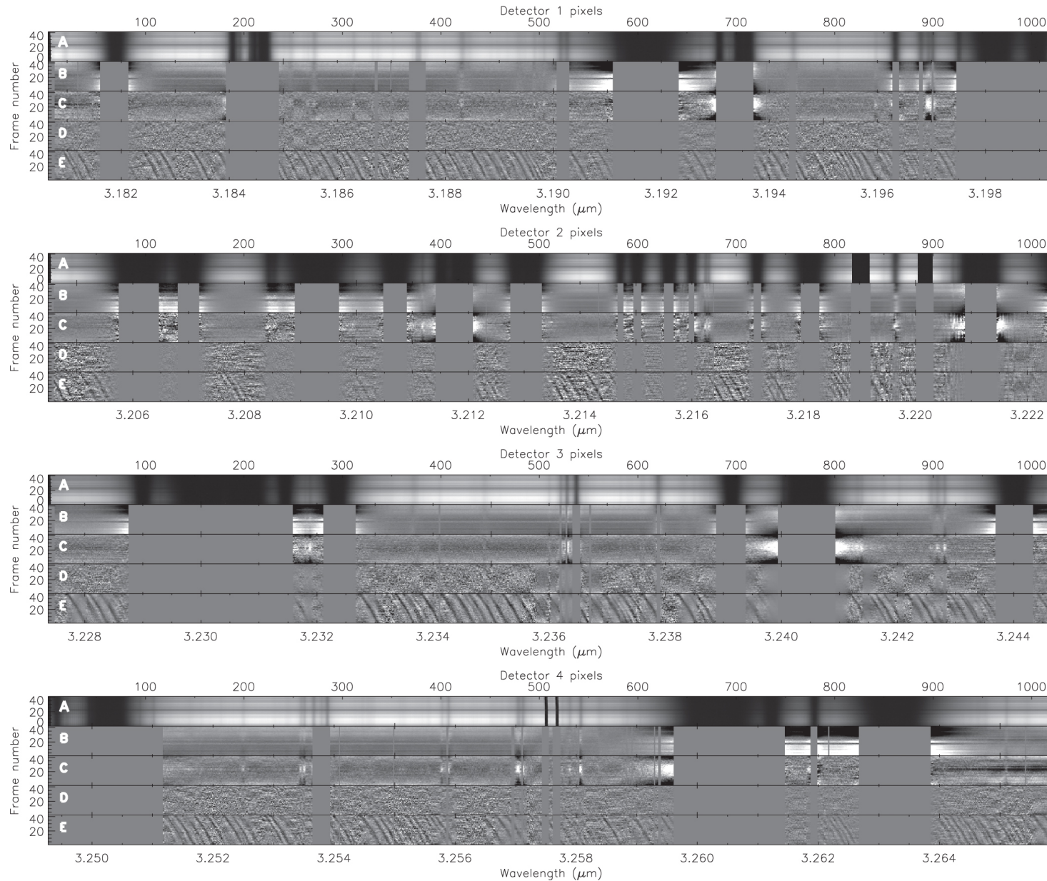
Figure 2. from Discovery of Water at High Spectral Resolution in the Atmosphere of 51 Peg b null 2017 AJ 153 138 doi:10.3847/1538-3881/aa5c87 https://dx.doi.org/10.3847/1538-3881/aa5c87 © 2017. The American Astronomical Society. All rights reserved.
