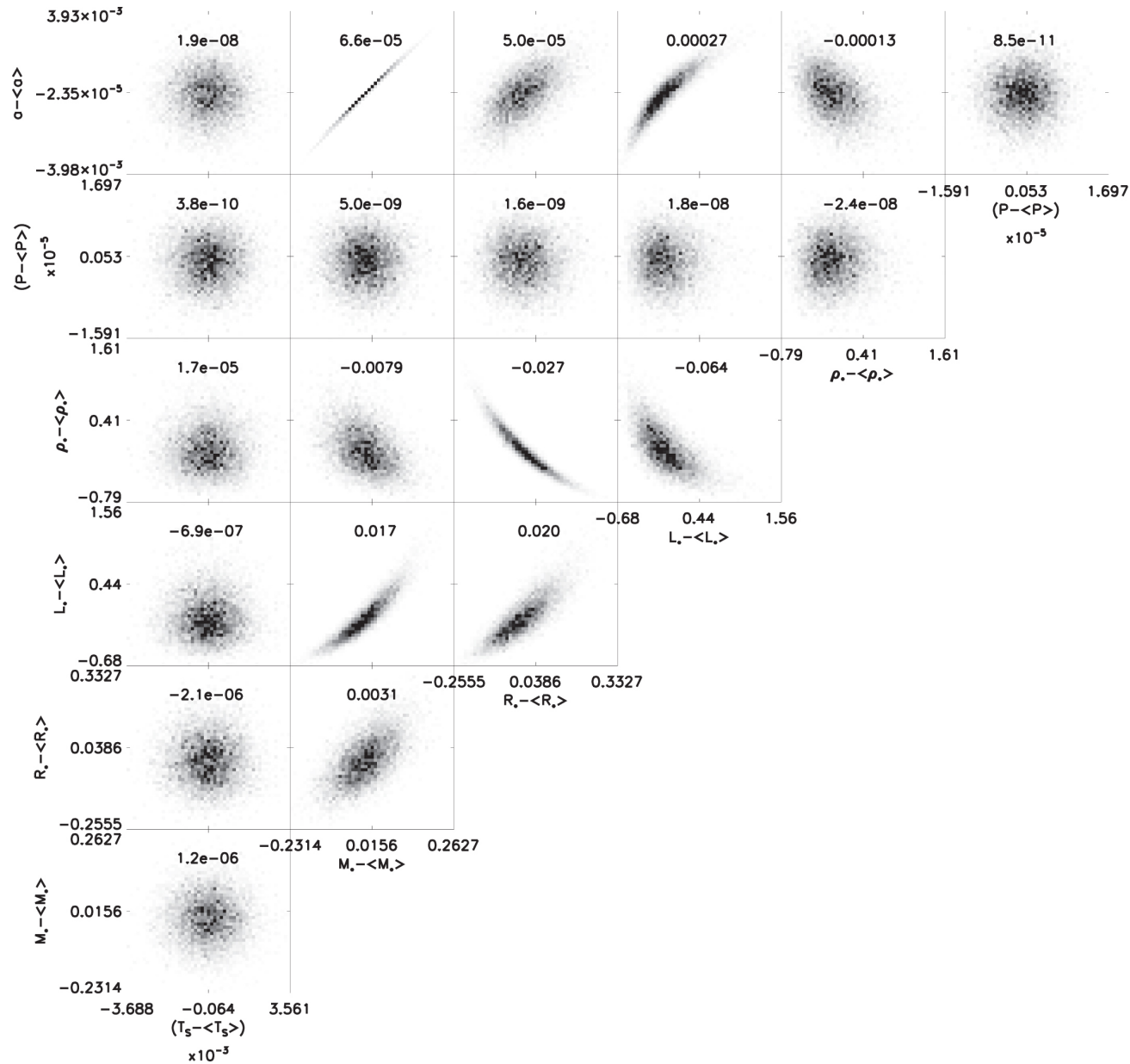
Figure 13. from Discovery of Water at High Spectral Resolution in the Atmosphere of 51 Peg b null 2017 AJ 153 138 doi:10.3847/1538-3881/aa5c87 https://dx.doi.org/10.3847/1538-3881/aa5c87
