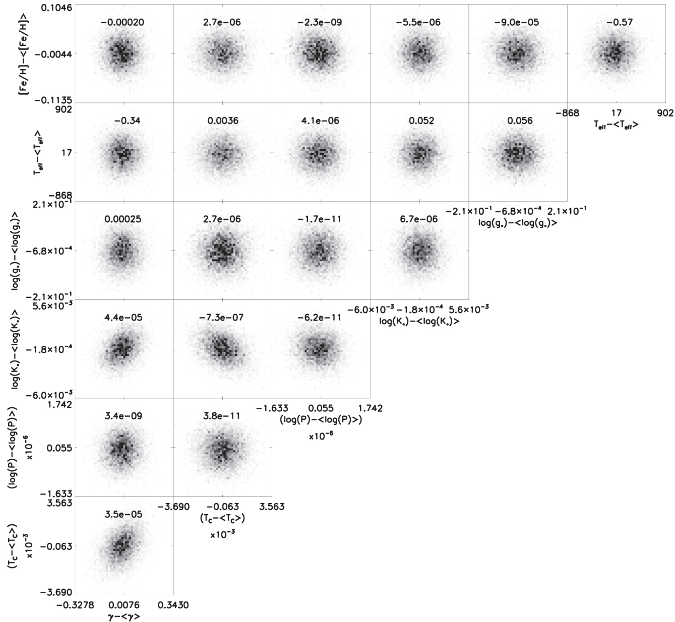
Figure 12. from Discovery of Water at High Spectral Resolution in the Atmosphere of 51 Peg b null 2017 AJ 153 138 doi:10.3847/1538-3881/aa5c87 https://dx.doi.org/10.3847/1538-3881/aa5c87
