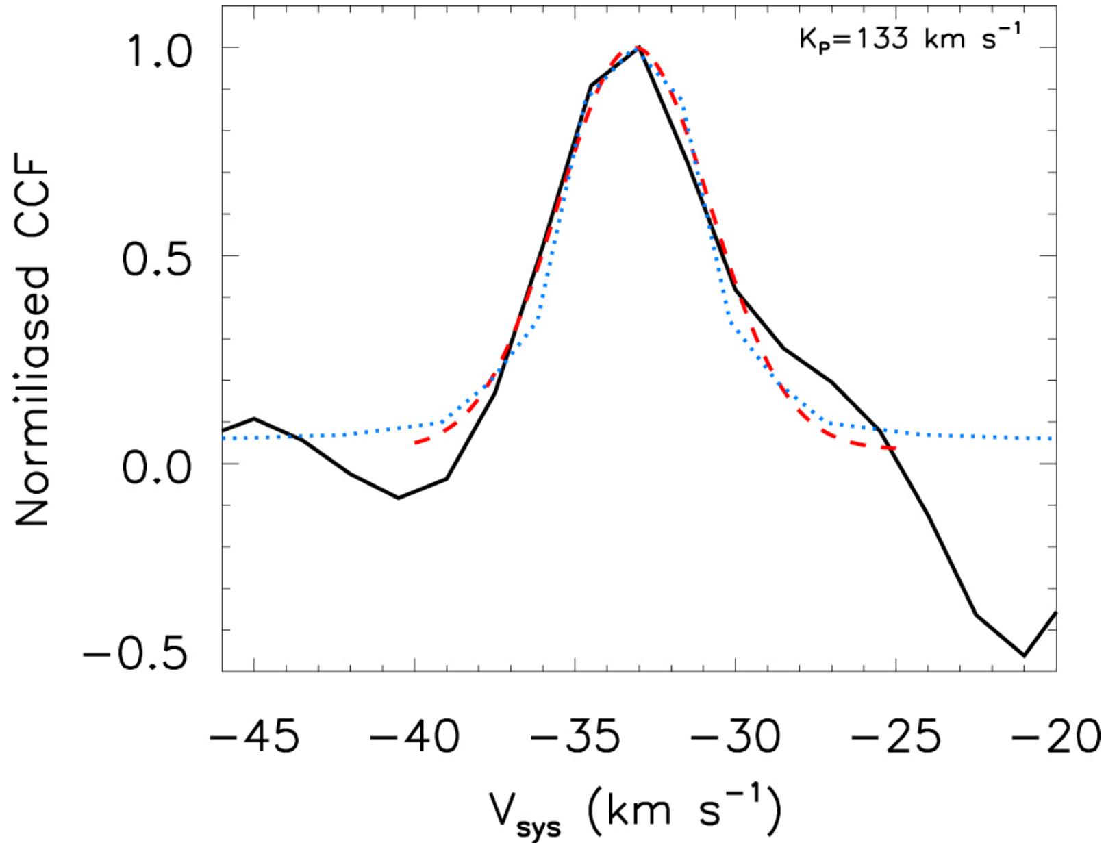
Figure 11. from Discovery of Water at High Spectral Resolution in the Atmosphere of 51 Peg b null 2017 AJ 153 138 doi:10.3847/1538-3881/aa5c87 https://dx.doi.org/10.3847/1538-3881/aa5c87 © 2017. The American Astronomical Society. All rights reserved.
