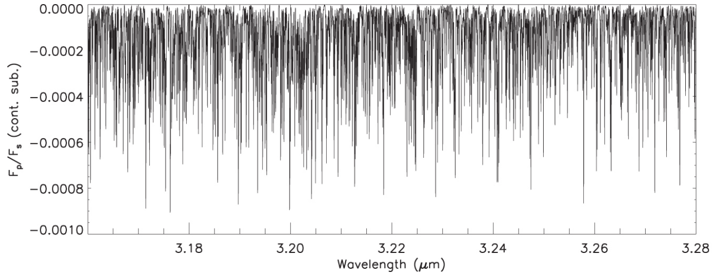
Figure 10. from Discovery of Water at High Spectral Resolution in the Atmosphere of 51 Peg b null 2017 AJ 153 138 doi:10.3847/1538-3881/aa5c87 https://dx.doi.org/10.3847/1538-3881/aa5c87
