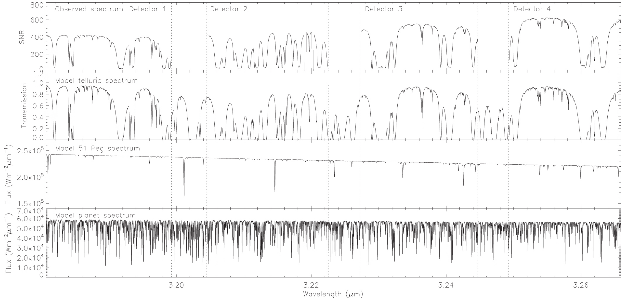
Figure 1. from Discovery of Water at High Spectral Resolution in the Atmosphere of 51 Peg b null 2017 AJ 153 138 doi:10.3847/1538-3881/aa5c87 https://dx.doi.org/10.3847/1538-3881/aa5c87 © 2017. The American Astronomical Society. All rights reserved.
