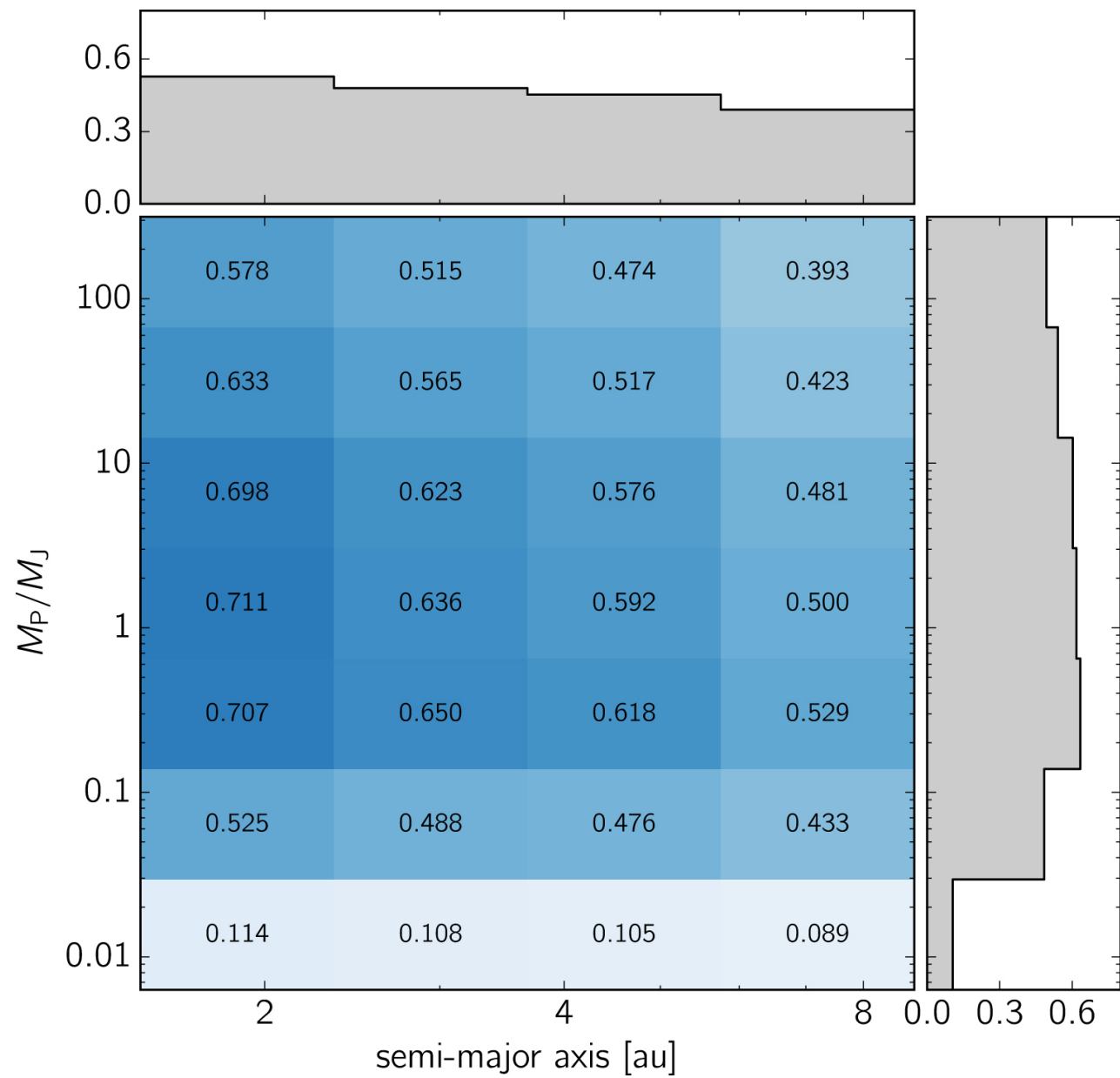
Figure 9. from THE POPULATION OF LONG-PERIOD TRANSITING EXOPLANETS null 2016 AJ 152 206 doi:10.3847/0004-6256/152/6/206 https://dx.doi.org/10.3847/0004-6256/152/6/206 © 2016. The American Astronomical Society. All rights reserved.
