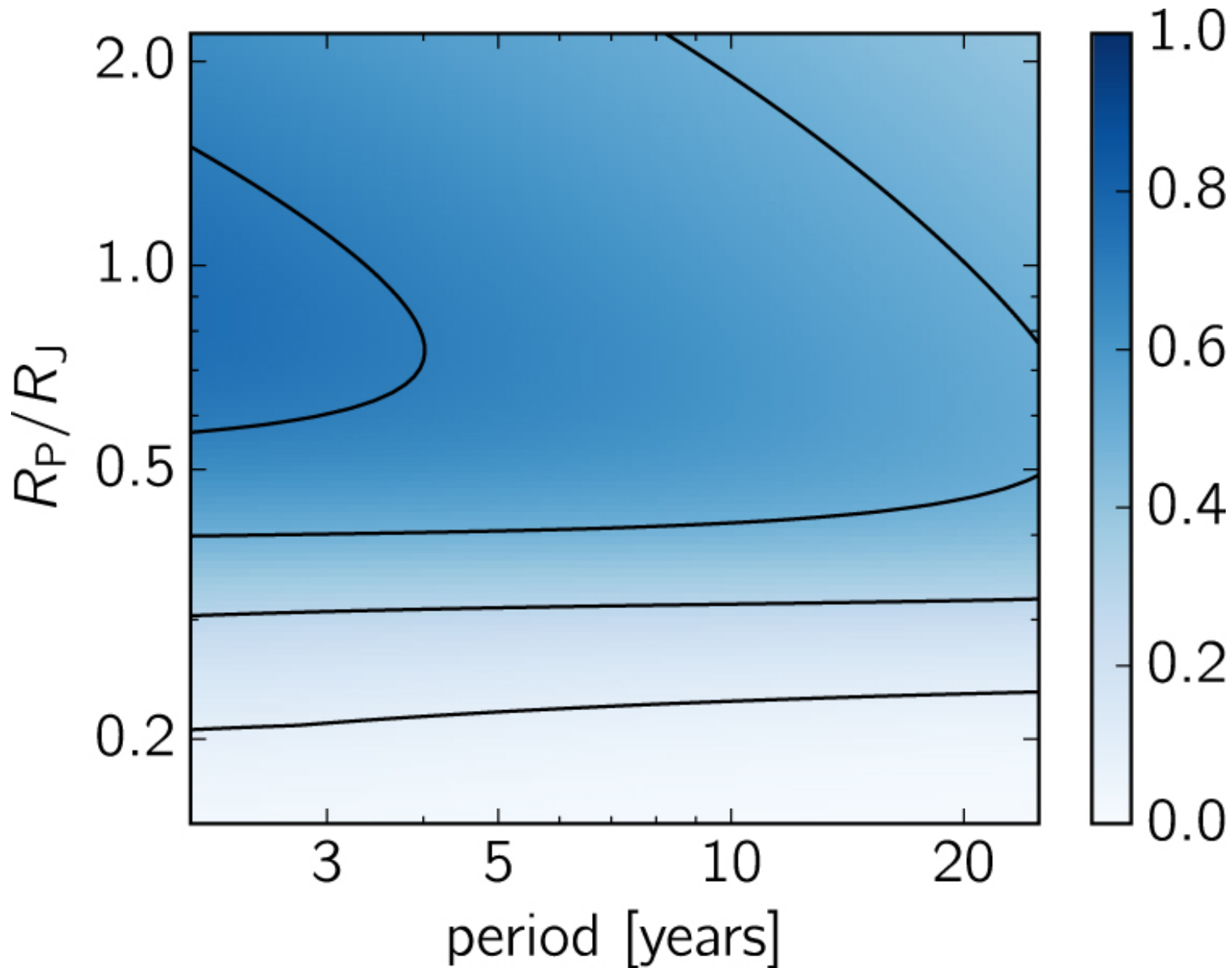
Figure 7. from THE POPULATION OF LONG-PERIOD TRANSITING EXOPLANETS null 2016 AJ 152 206 doi:10.3847/0004-6256/152/6/206 https://dx.doi.org/10.3847/0004-6256/152/6/206 © 2016. The American Astronomical Society. All rights reserved.
