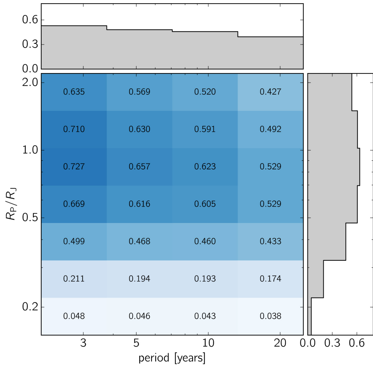
Figure 6. from THE POPULATION OF LONG-PERIOD TRANSITING EXOPLANETS null 2016 AJ 152 206 doi:10.3847/0004-6256/152/6/206 https://dx.doi.org/10.3847/0004-6256/152/6/206 © 2016. The American Astronomical Society. All rights reserved.
