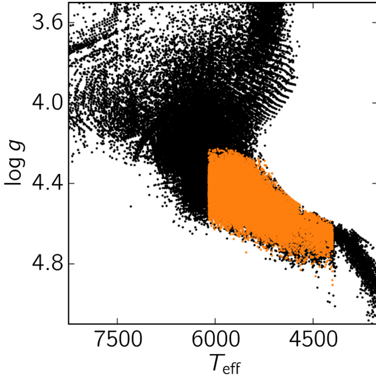
Figure 2. from THE POPULATION OF LONG-PERIOD TRANSITING EXOPLANETS null 2016 AJ 152 206 doi:10.3847/0004-6256/152/6/206 https://dx.doi.org/10.3847/0004-6256/152/6/206 © 2016. The American Astronomical Society. All rights reserved.
