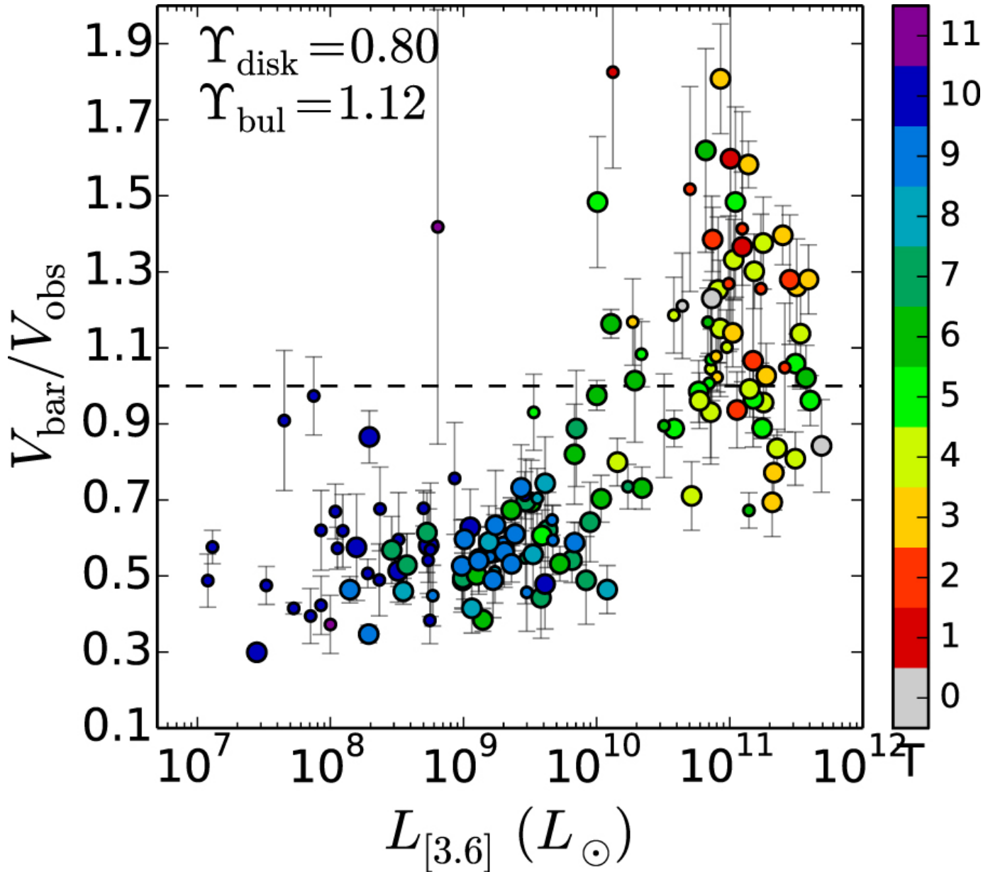
Figure 8. from SPARC: MASS MODELS FOR 175 DISK GALAXIES WITH SPITZER PHOTOMETRY AND ACCURATE ROTATION CURVES null 2016 AJ 152 157 doi:10.3847/0004-6256/152/6/157 https://dx.doi.org/10.3847/0004-6256/152/6/157 © 2016. The American Astronomical Society. All rights reserved.
