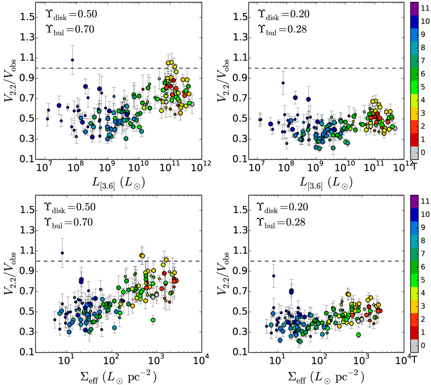
Figure 6. from SPARC: MASS MODELS FOR 175 DISK GALAXIES WITH SPITZER PHOTOMETRY AND ACCURATE ROTATION CURVES null 2016 AJ 152 157 doi:10.3847/0004-6256/152/6/157 https://dx.doi.org/10.3847/0004-6256/152/6/157 © 2016. The American Astronomical Society. All rights reserved.
