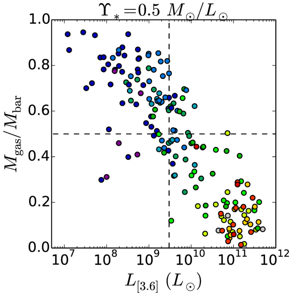
Figure 4. from SPARC: MASS MODELS FOR 175 DISK GALAXIES WITH SPITZER PHOTOMETRY AND ACCURATE ROTATION CURVES null 2016 AJ 152 157 doi:10.3847/0004-6256/152/6/157 https://dx.doi.org/10.3847/0004-6256/152/6/157 © 2016. The American Astronomical Society. All rights reserved.
