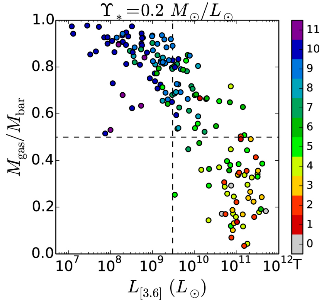
Figure 4. from SPARC: MASS MODELS FOR 175 DISK GALAXIES WITH SPITZER PHOTOMETRY AND ACCURATE ROTATION CURVES null 2016 AJ 152 157 doi:10.3847/0004-6256/152/6/157 https://dx.doi.org/10.3847/0004-6256/152/6/157 © 2016. The American Astronomical Society. All rights reserved.
