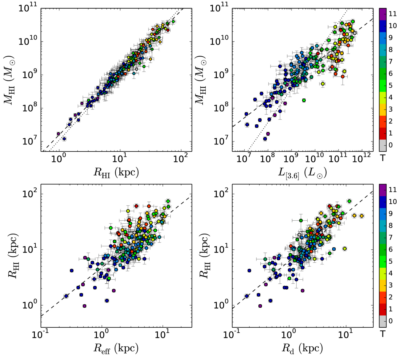
Figure 3. from SPARC: MASS MODELS FOR 175 DISK GALAXIES WITH SPITZER PHOTOMETRY AND ACCURATE ROTATION CURVES null 2016 AJ 152 157 doi:10.3847/0004-6256/152/6/157 https://dx.doi.org/10.3847/0004-6256/152/6/157
