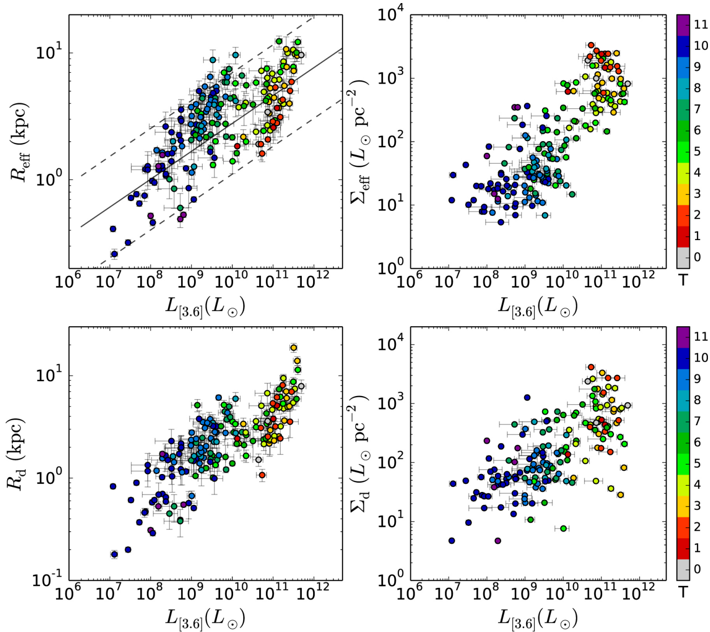
Figure 2. from SPARC: MASS MODELS FOR 175 DISK GALAXIES WITH SPITZER PHOTOMETRY AND ACCURATE ROTATION CURVES null 2016 AJ 152 157 doi:10.3847/0004-6256/152/6/157 https://dx.doi.org/10.3847/0004-6256/152/6/157 © 2016. The American Astronomical Society. All rights reserved.
