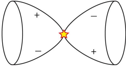
Figure 9. from NEAR-INFRARED CIRCULAR AND LINEAR POLARIMETRY OF MONOCEROS R2 null 2016 AJ 152 67 doi:10.3847/0004-6256/152/3/67 https://dx.doi.org/10.3847/0004-6256/152/3/67 © 2016. The American Astronomical Society. All rights reserved.
