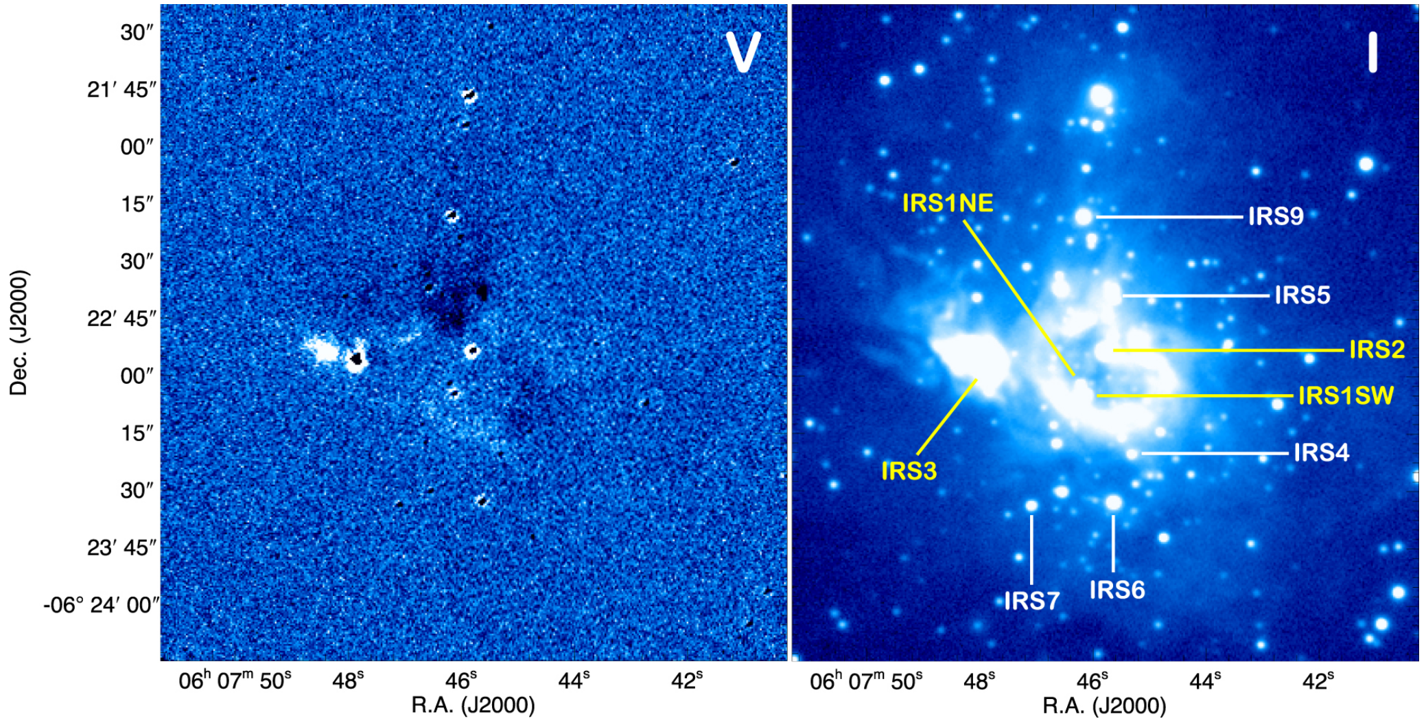
Figure 8. from NEAR-INFRARED CIRCULAR AND LINEAR POLARIMETRY OF MONOCEROS R2 null 2016 AJ 152 67 doi:10.3847/0004-6256/152/3/67 https://dx.doi.org/10.3847/0004-6256/152/3/67 © 2016. The American Astronomical Society. All rights reserved.
