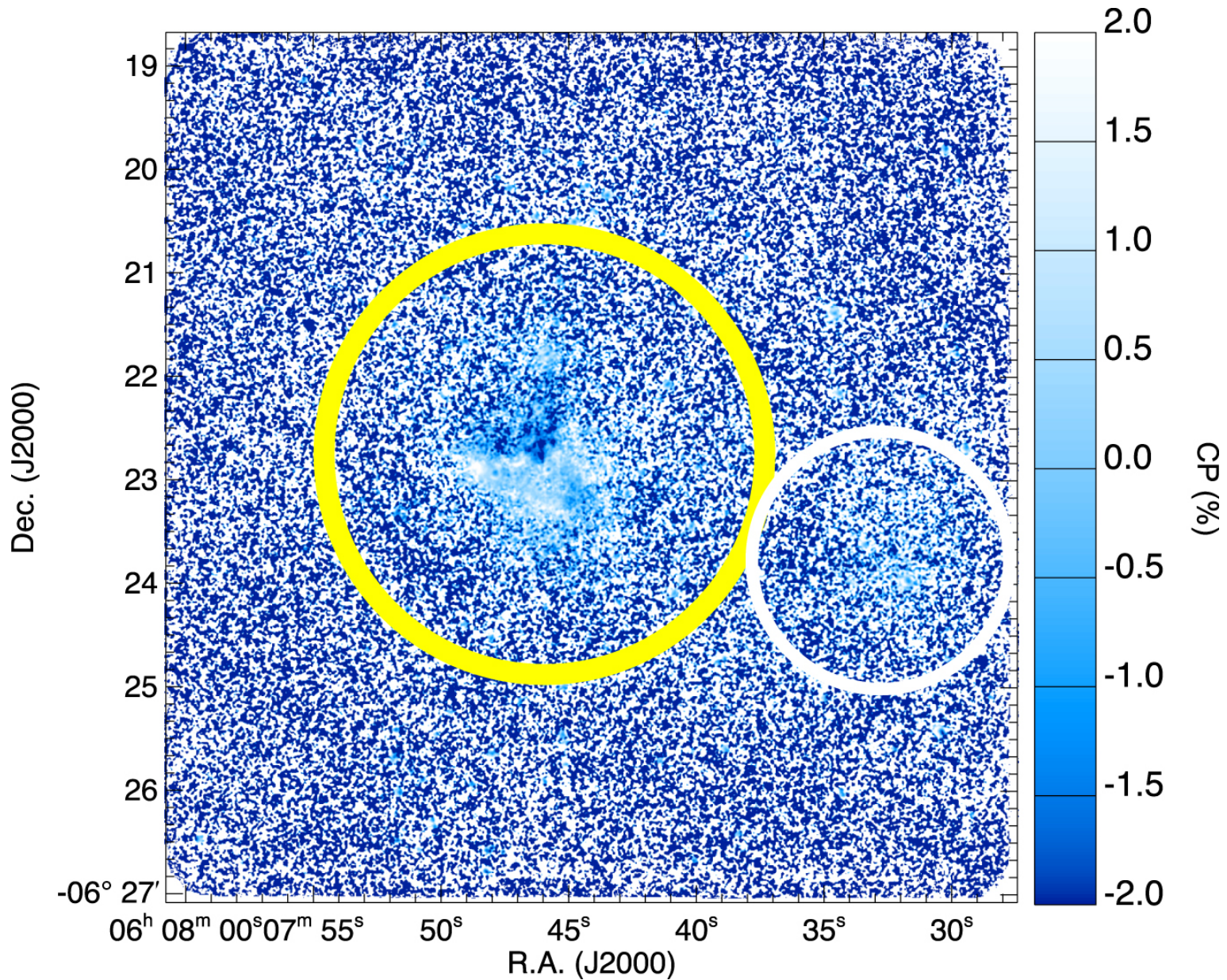
Figure 7. from NEAR-INFRARED CIRCULAR AND LINEAR POLARIMETRY OF MONOCEROS R2 null 2016 AJ 152 67 doi:10.3847/0004-6256/152/3/67 https://dx.doi.org/10.3847/0004-6256/152/3/67 © 2016. The American Astronomical Society. All rights reserved.
