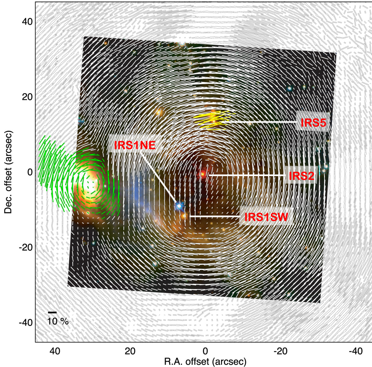
Figure 6. from NEAR-INFRARED CIRCULAR AND LINEAR POLARIMETRY OF MONOCEROS R2 null 2016 AJ 152 67 doi:10.3847/0004-6256/152/3/67 https://dx.doi.org/10.3847/0004-6256/152/3/67 © 2016. The American Astronomical Society. All rights reserved.
