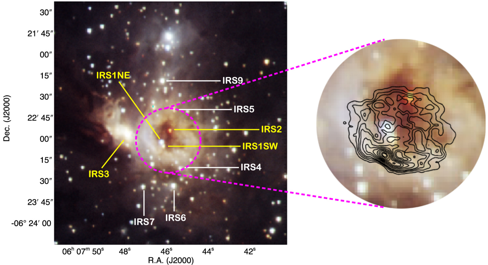
Figure 2. from NEAR-INFRARED CIRCULAR AND LINEAR POLARIMETRY OF MONOCEROS R2 null 2016 AJ 152 67 doi:10.3847/0004-6256/152/3/67 https://dx.doi.org/10.3847/0004-6256/152/3/67 © 2016. The American Astronomical Society. All rights reserved.
