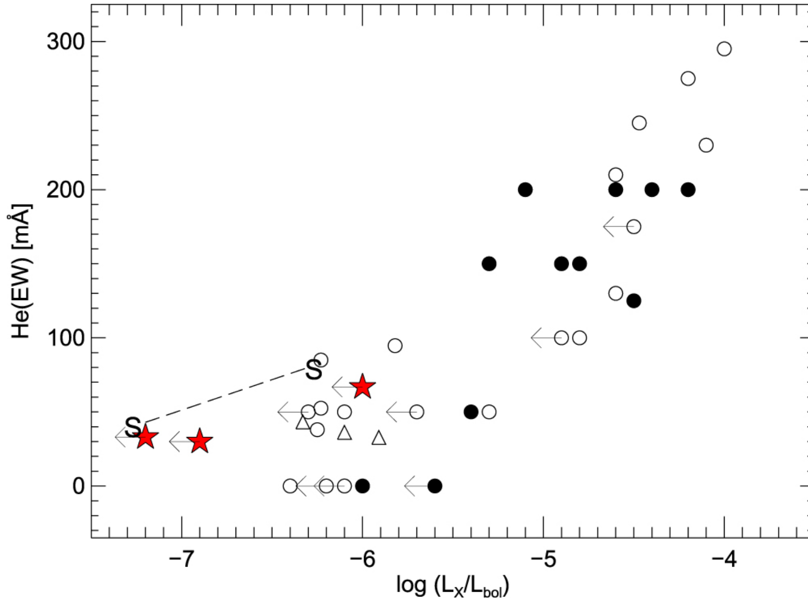
Figure 3. from A SEARCH FOR CORONAL ACTIVITY AMONG TWO METAL-POOR SUBDWARFS AND ONE SUBGIANT null 2016 AJ 152 43 doi:10.3847/0004-6256/152/2/43 https://dx.doi.org/10.3847/0004-6256/152/2/43 © 2016. The American Astronomical Society. All rights reserved.
