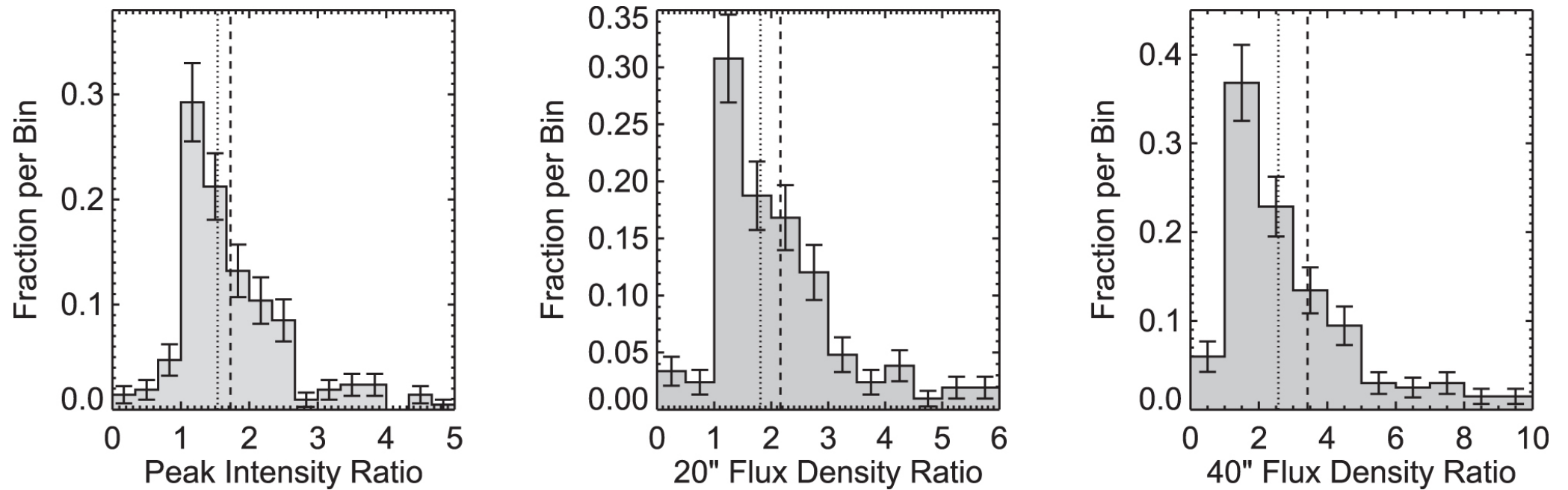
Figure 9. from A CATALOG OF LOW-MASS STAR-FORMING CORES OBSERVED WITH SHARC-II AT 350 \mu m null 2016 AJ 152 36 doi:10.3847/0004-6256/152/2/36 https://dx.doi.org/10.3847/0004-6256/152/2/36 © 2016. The American Astronomical Society. All rights reserved.
