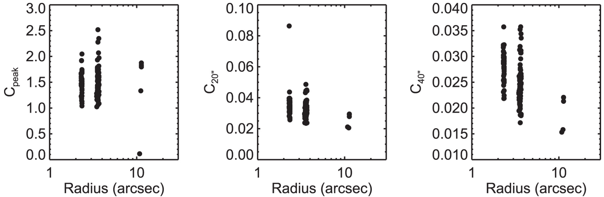
Figure 5. from A CATALOG OF LOW-MASS STAR-FORMING CORES OBSERVED WITH SHARC-II AT 350 m null 2016 AJ 152 36 doi:10.3847/0004-6256/152/2/36 https://dx.doi.org/10.3847/0004-6256/152/2/36
