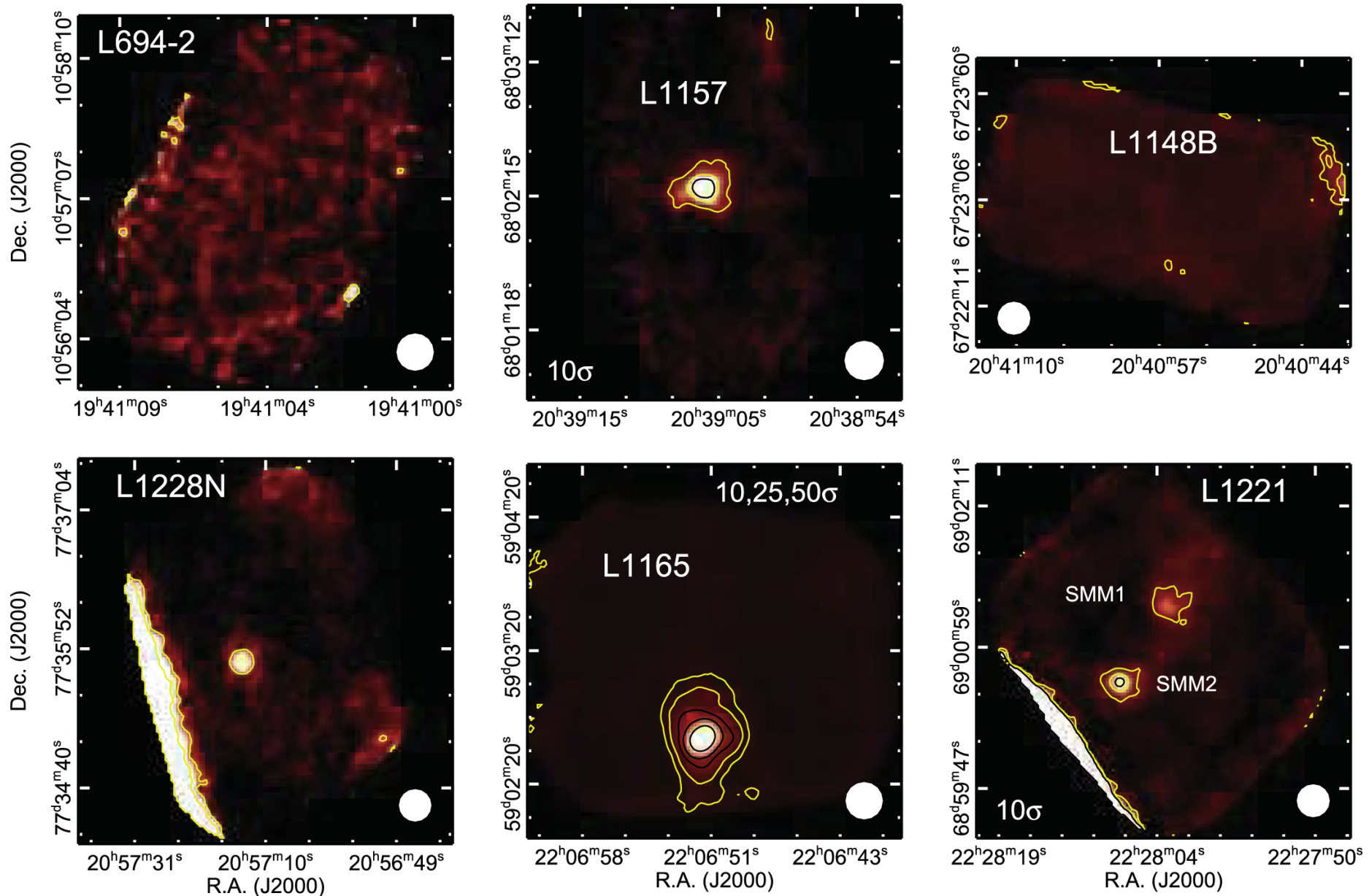
Figure 35. from A CATALOG OF LOW-MASS STAR-FORMING CORES OBSERVED WITH SHARC-II AT 350 m null 2016 AJ 152 36 doi:10.3847/0004-6256/152/2/36 https://dx.doi.org/10.3847/0004-6256/152/2/36 © 2016. The American Astronomical Society. All rights reserved.
