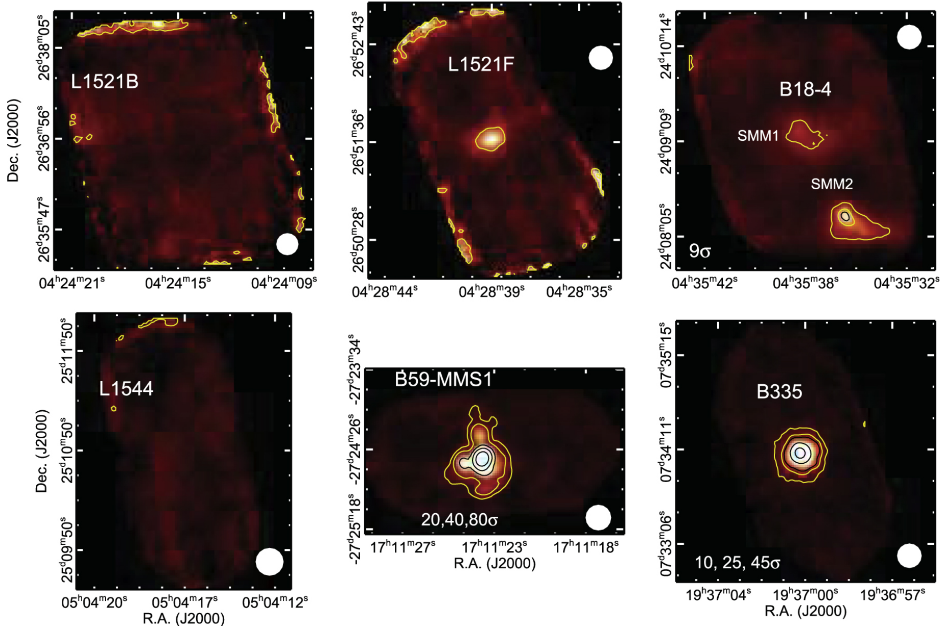
Figure 34. from A CATALOG OF LOW-MASS STAR-FORMING CORES OBSERVED WITH SHARC-II AT 350 m null 2016 AJ 152 36 doi:10.3847/0004-6256/152/2/36 https://dx.doi.org/10.3847/0004-6256/152/2/36 © 2016. The American Astronomical Society. All rights reserved.
